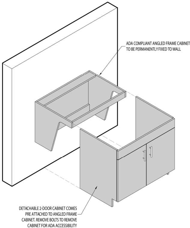
1 ISOMETRIC - ISOMETRIC - ADA COMPLIANT CABINET WITH REMOVABLE 2 DOOR SHROUD SCALE: RE:
