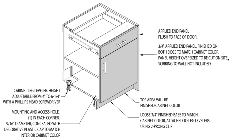
3 ISOMETRIC - CABINET LEG LEVELER DETAIL SCALE: RE:
