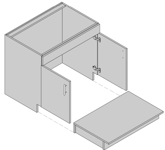
2 ISOMETRIC - 2 DOOR ADA SINK BASE WITH REMOVABLE PEDESTAL SCALE: RE:
