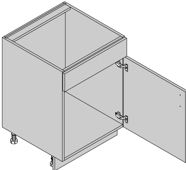
Base 1 Door False Front Sink Right
